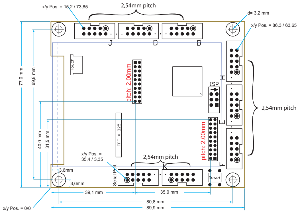
PCB: component side
